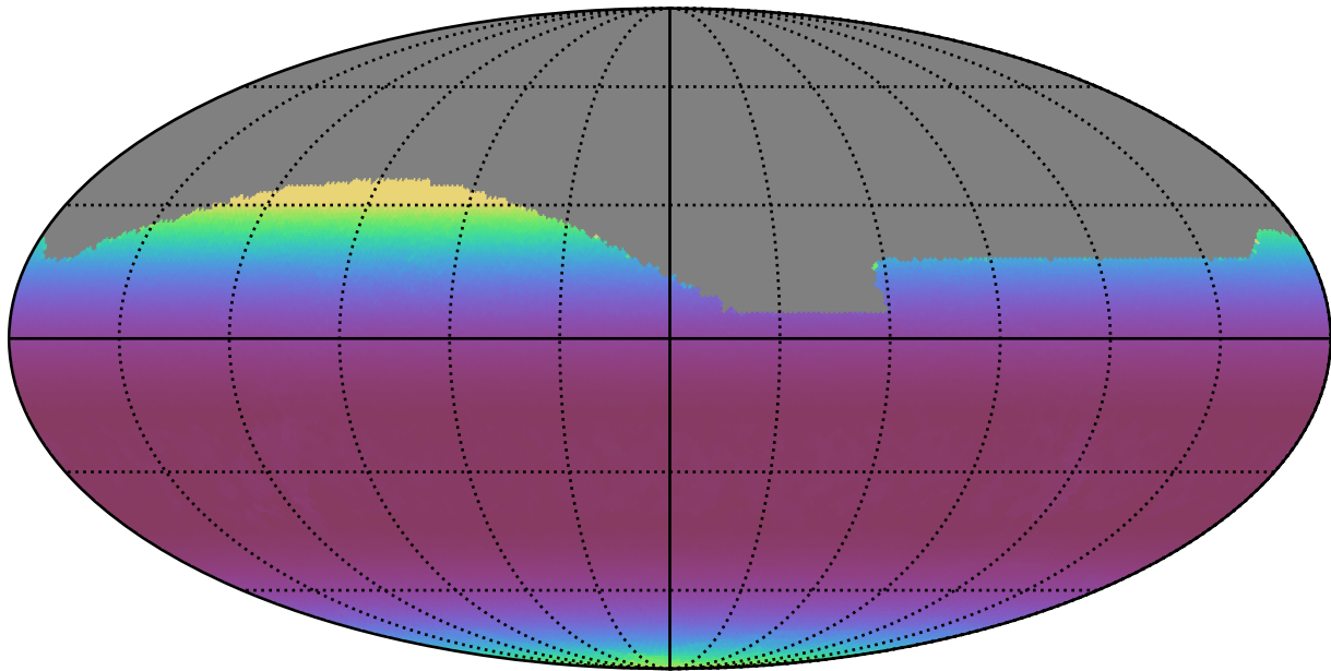
ddf_loaded_fl8_v3.4_10yrs All sky i band: Min airmass
