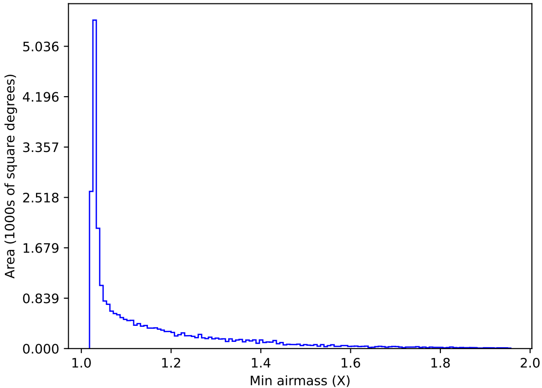
ddf_loaded_fl8_v3.4_10yrs All sky i band: Min airmass
