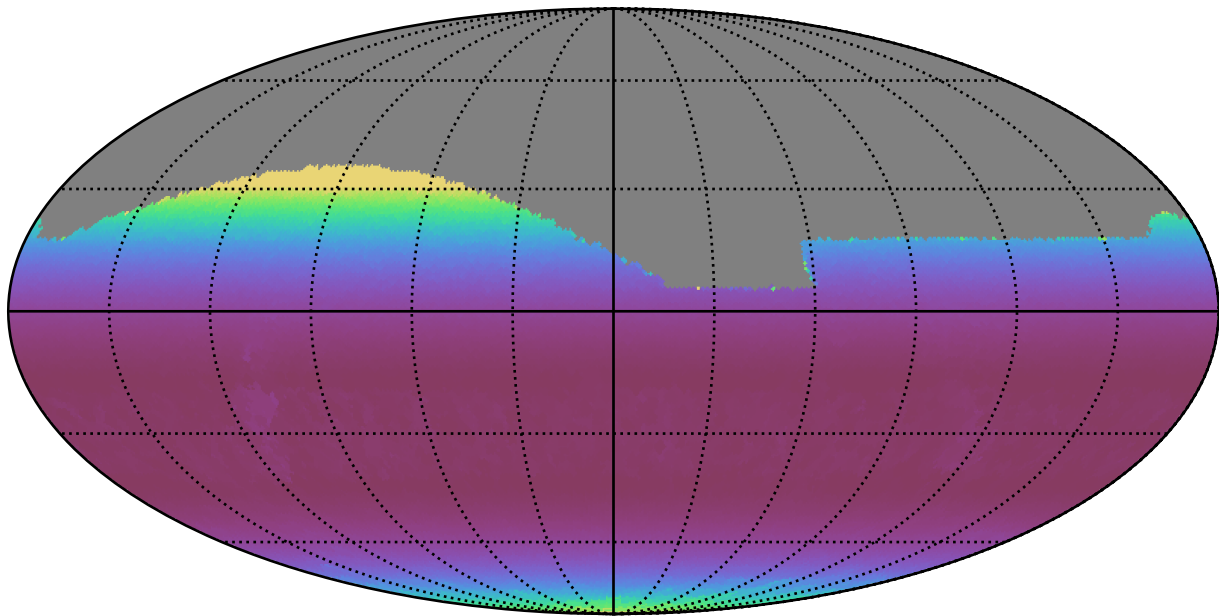
ddf_loaded_fl8_v3.4_10yrs All sky g band: Min airmass
