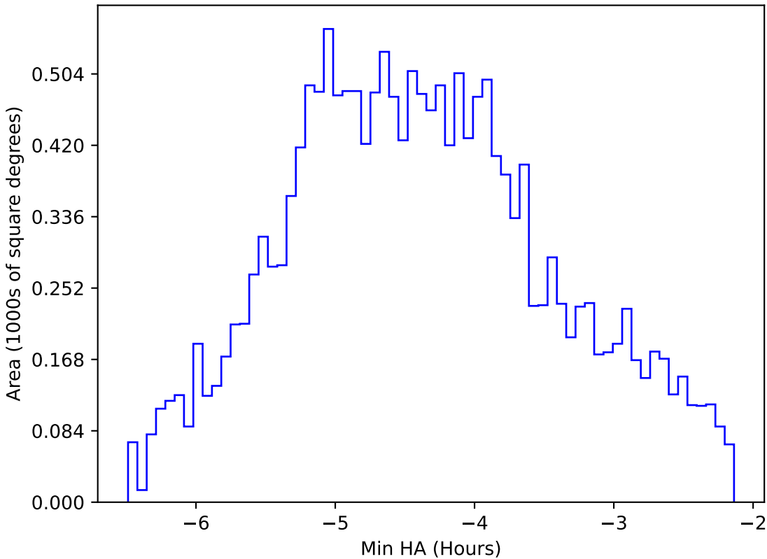
ddf_loaded_fl8_v3.4_10yrs WFD z band: Min HA
