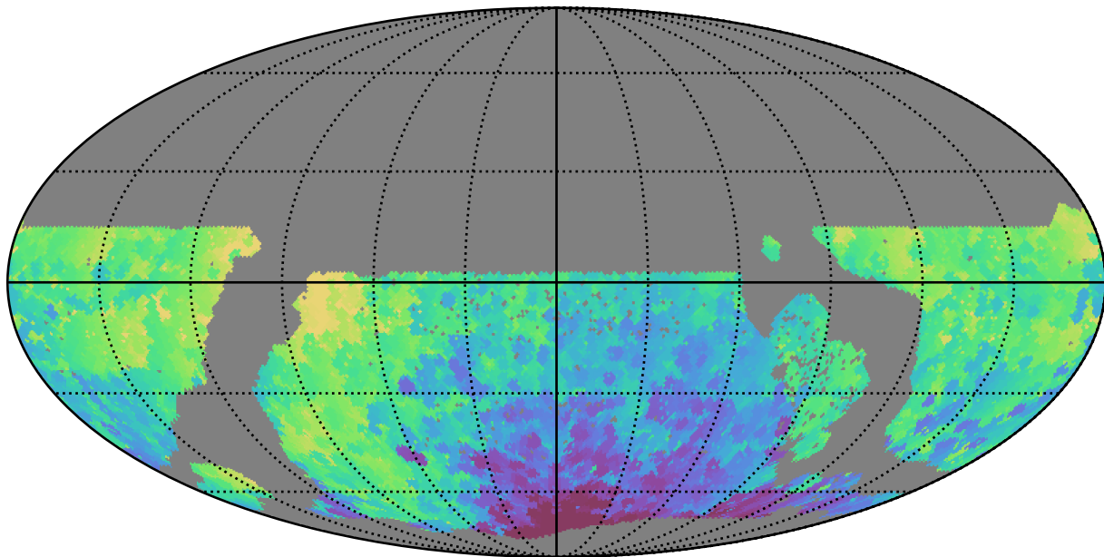
ddf_loaded_fl8_v3.4_10yrs WFD y band: Min HA
