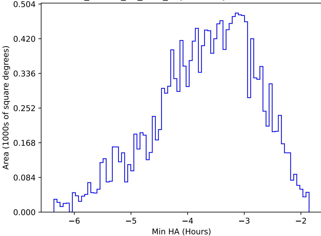
ddf_loaded_fl8_v3.4_10yrs WFD y band: Min HA
