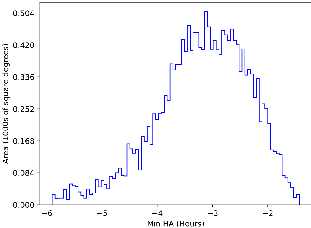
ddf_loaded_fl8_v3.4_10yrs WFD u band: Min HA
