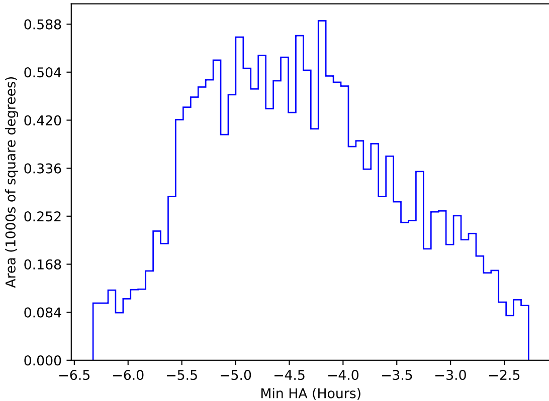
ddf_loaded_fl8_v3.4_10yrs WFD r band: Min HA
