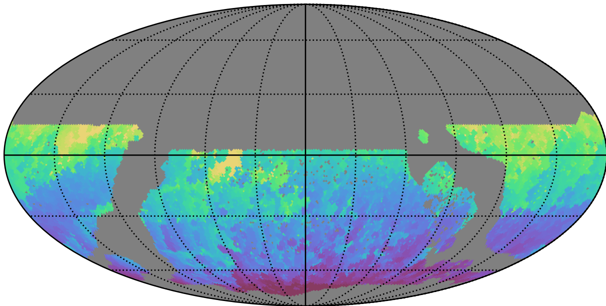
ddf_loaded_fl8_v3.4_10yrs WFD i band: Min HA
