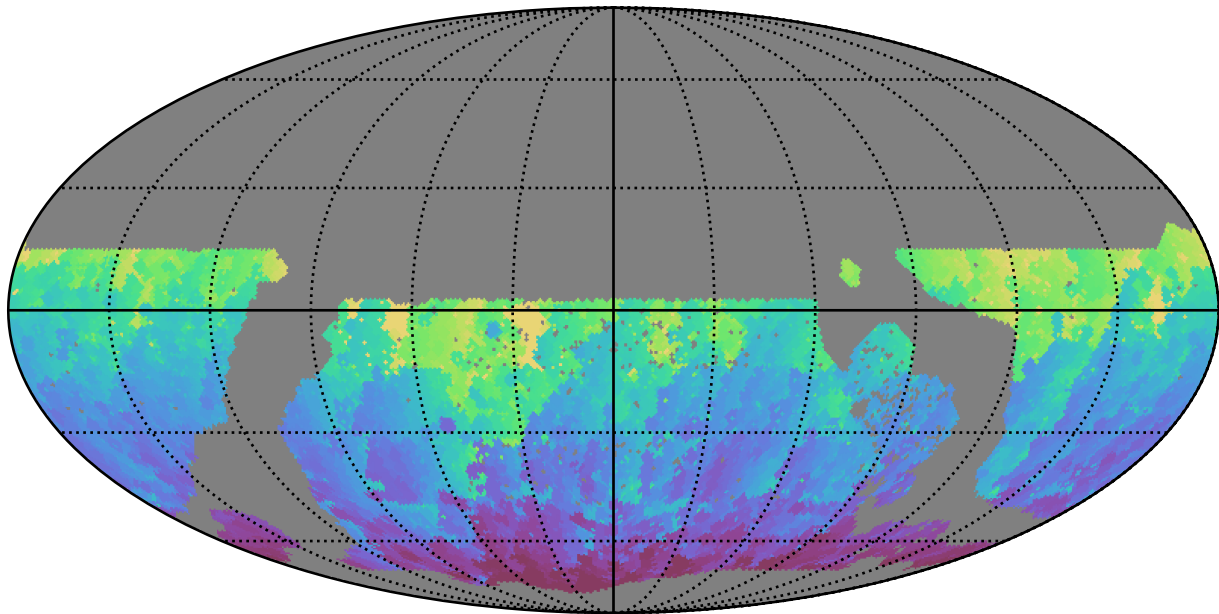
ddf_loaded_fl8_v3.4_10yrs WFD g band: Min HA
