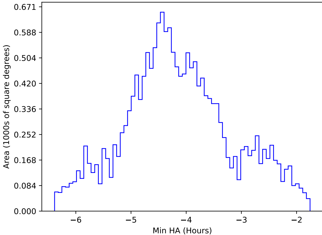
ddf_loaded_fl8_v3.4_10yrs WFD g band: Min HA
