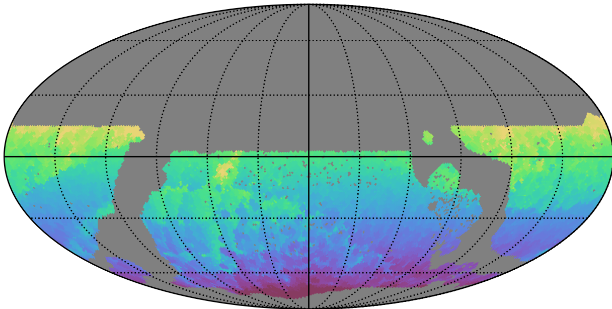
ddf_loaded_fl8_v3.4_10yrs WFD all bands: Min HA
