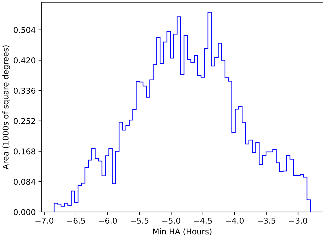
ddf_loaded_fl8_v3.4_10yrs WFD all bands: Min HA
