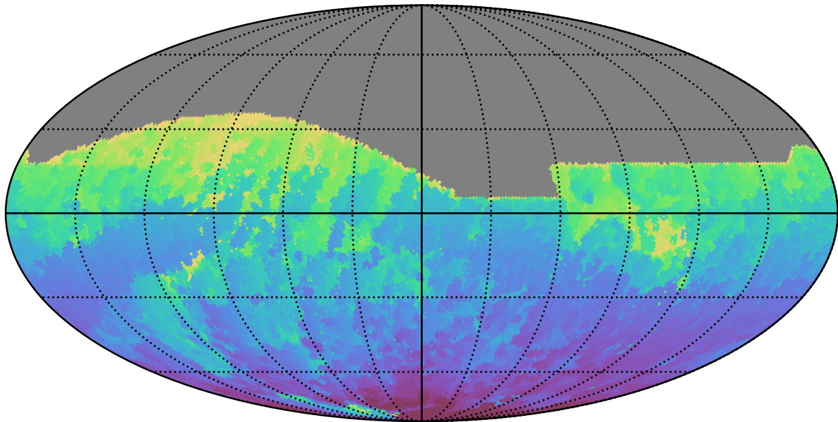
ddf_loaded_fl8_v3.4_10yrs All sky z band: Min HA
