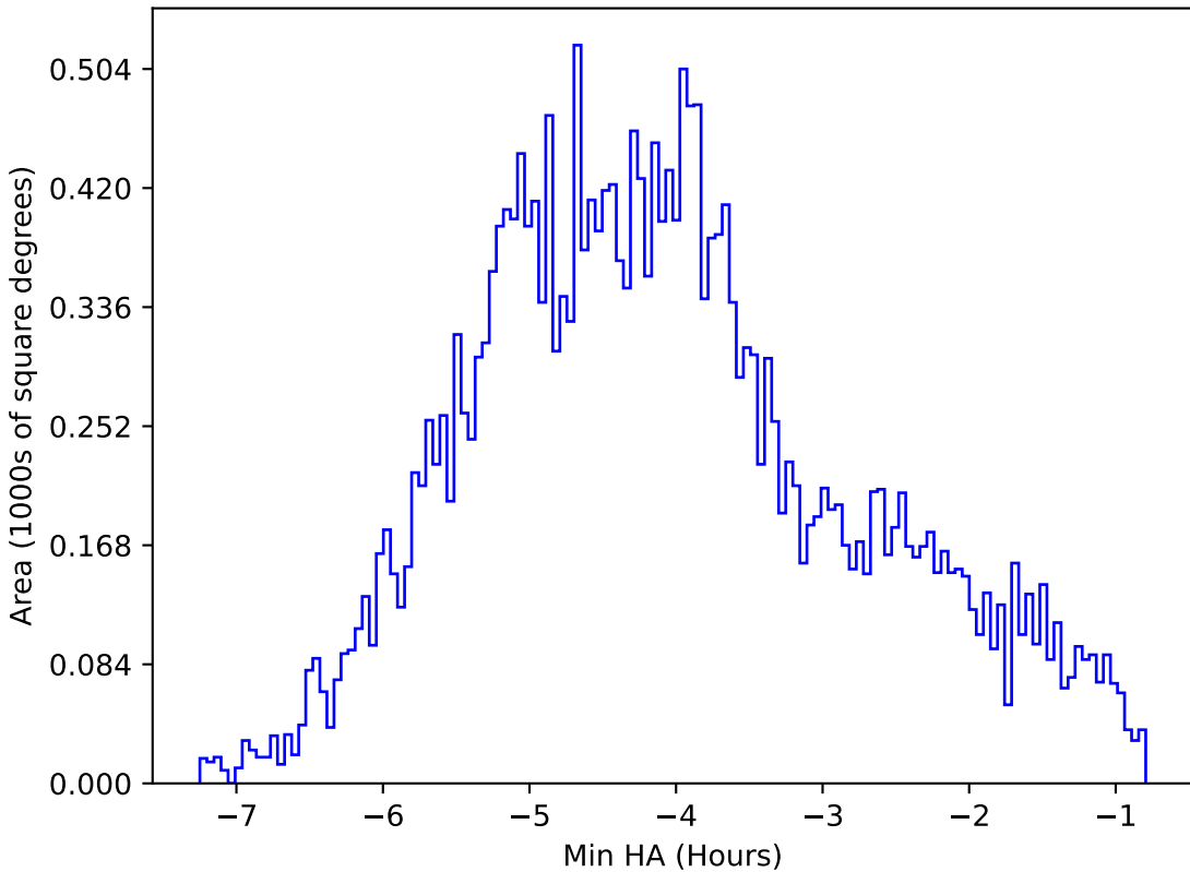
ddf_loaded_fl8_v3.4_10yrs All sky z band: Min HA
