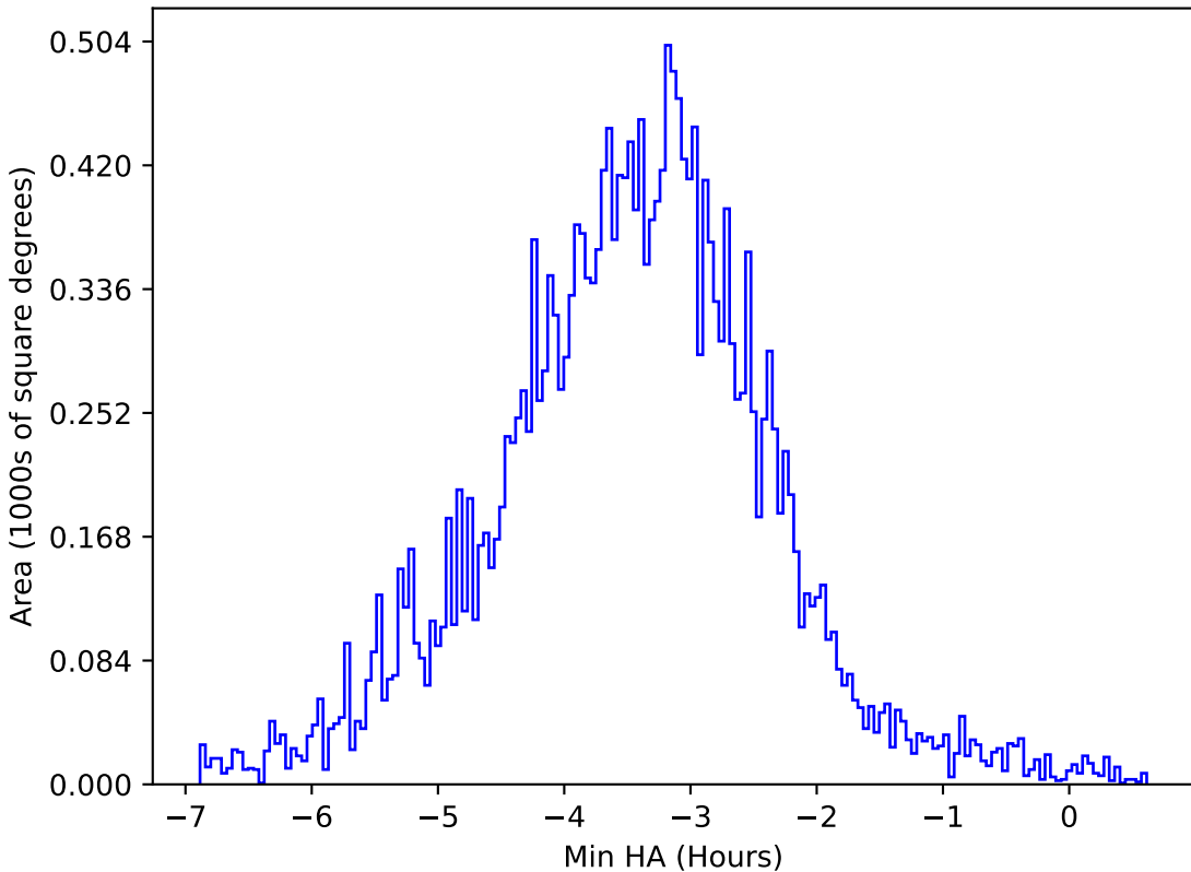
ddf_loaded_fl8_v3.4_10yrs All sky y band: Min HA
