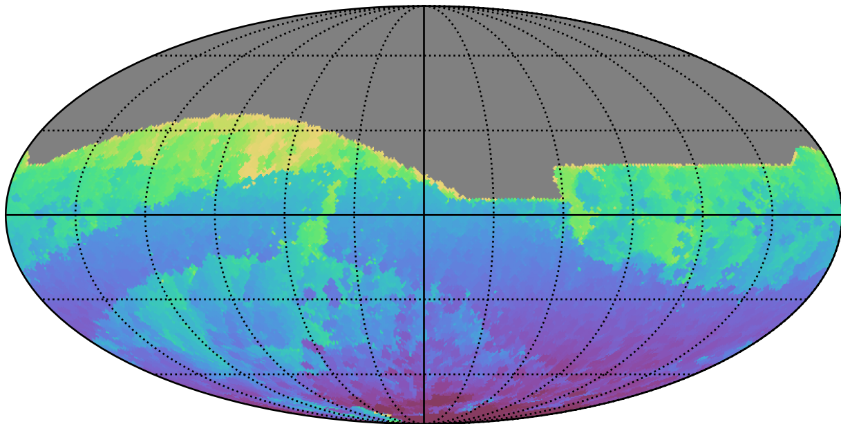
ddf_loaded_fl8_v3.4_10yrs All sky r band: Min HA
