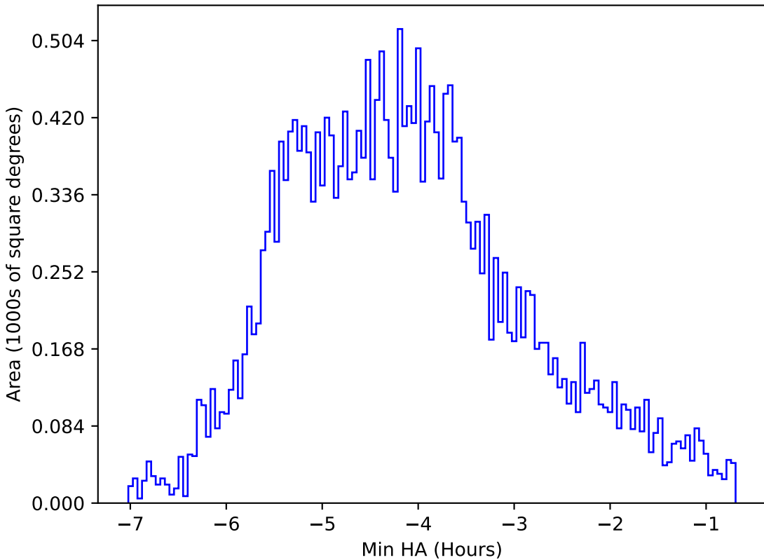
ddf_loaded_fl8_v3.4_10yrs All sky r band: Min HA
