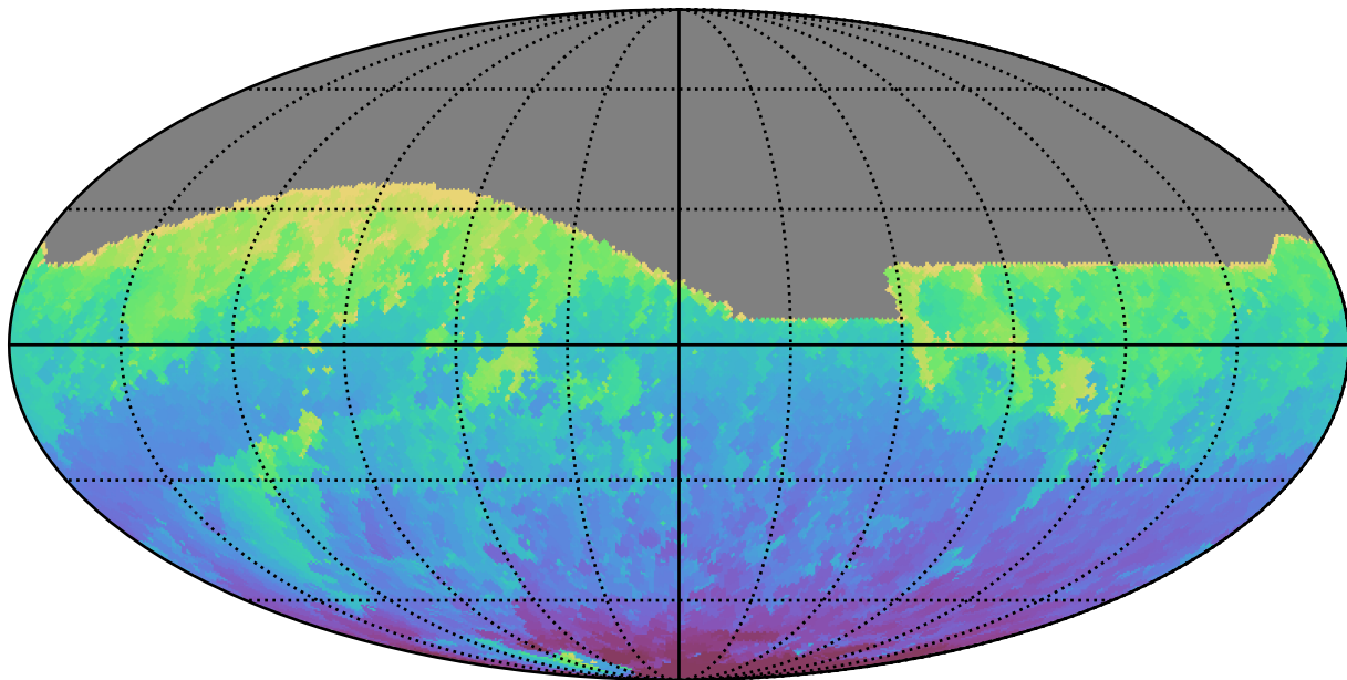
ddf_loaded_fl8_v3.4_10yrs All sky i band: Min HA
