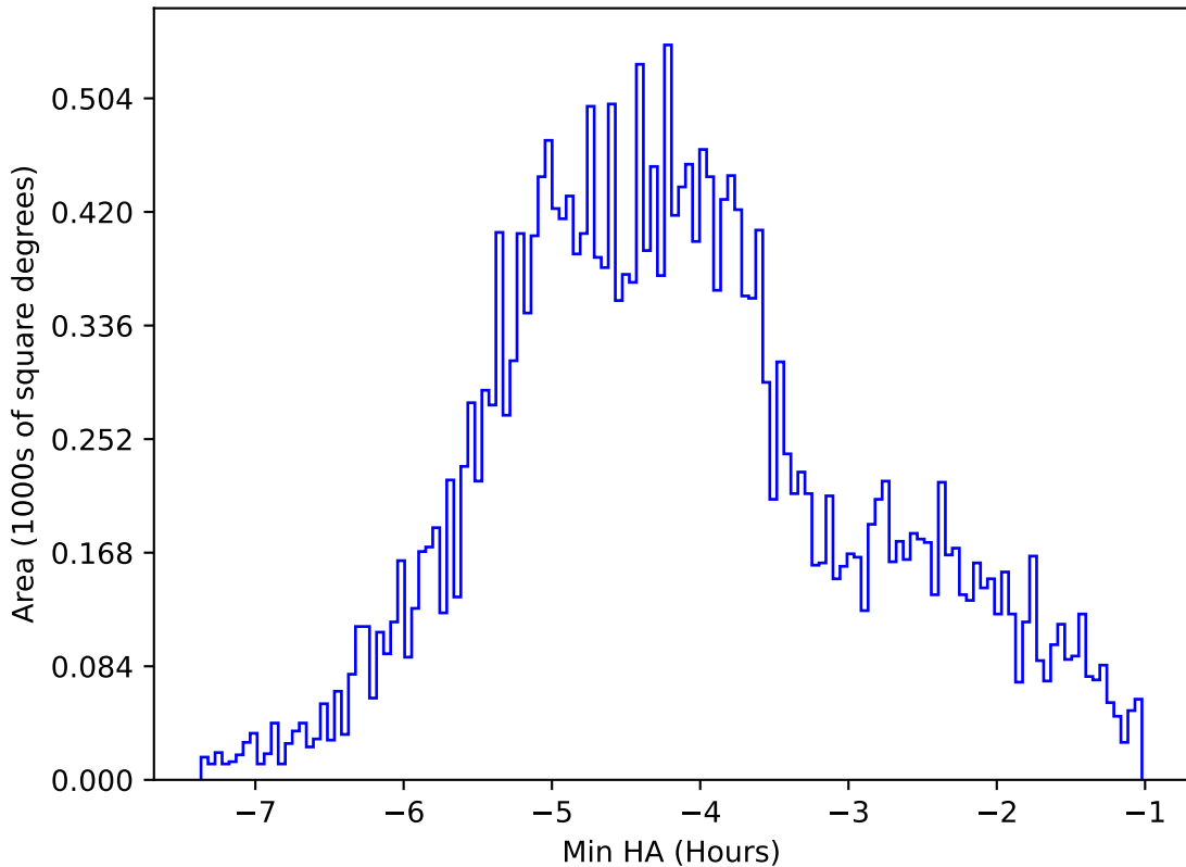
ddf_loaded_fl8_v3.4_10yrs All sky i band: Min HA
