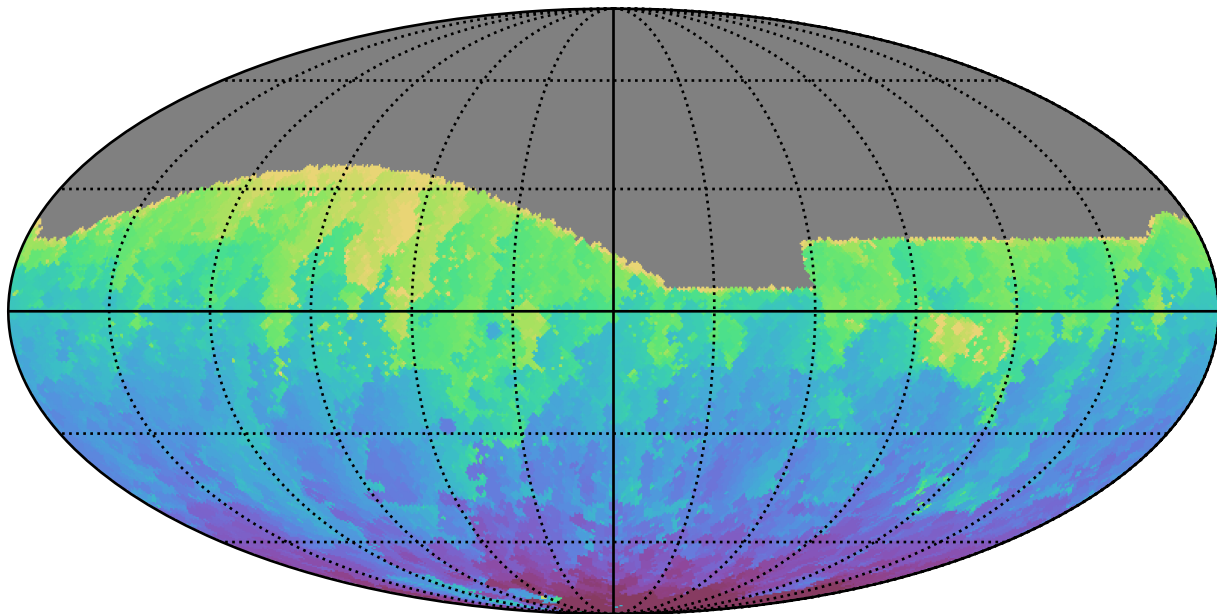
ddf_loaded_fl8_v3.4_10yrs All sky g band: Min HA
