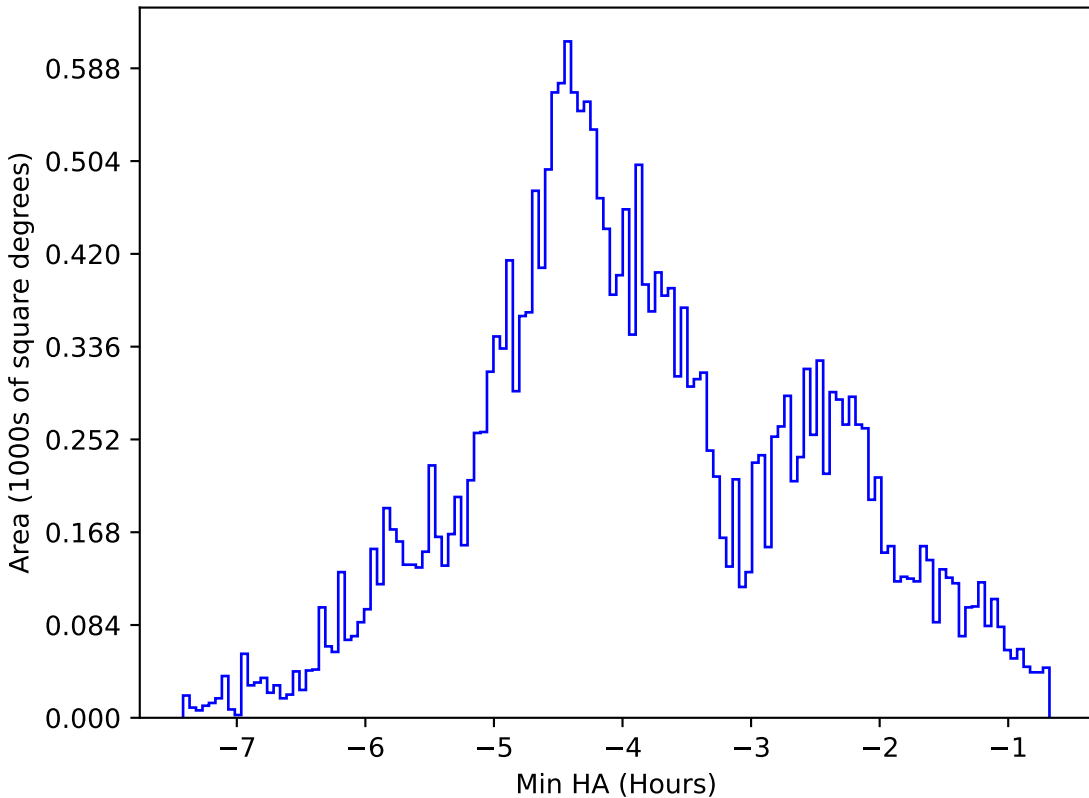
ddf_loaded_fl8_v3.4_10yrs All sky g band: Min HA
