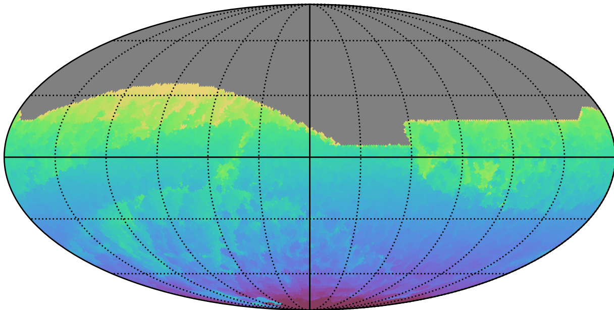
ddf_loaded_fl8_v3.4_10yrs All sky all bands: Min HA
