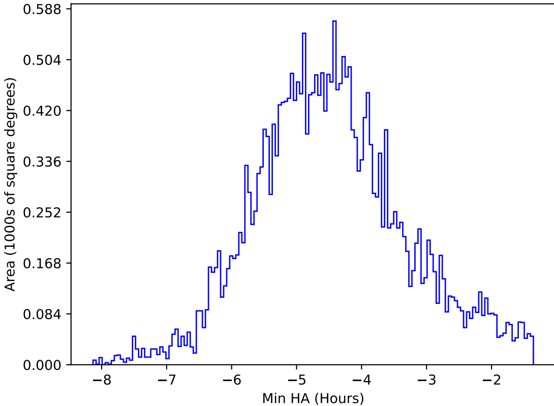
ddf_loaded_fl8_v3.4_10yrs All sky all bands: Min HA
