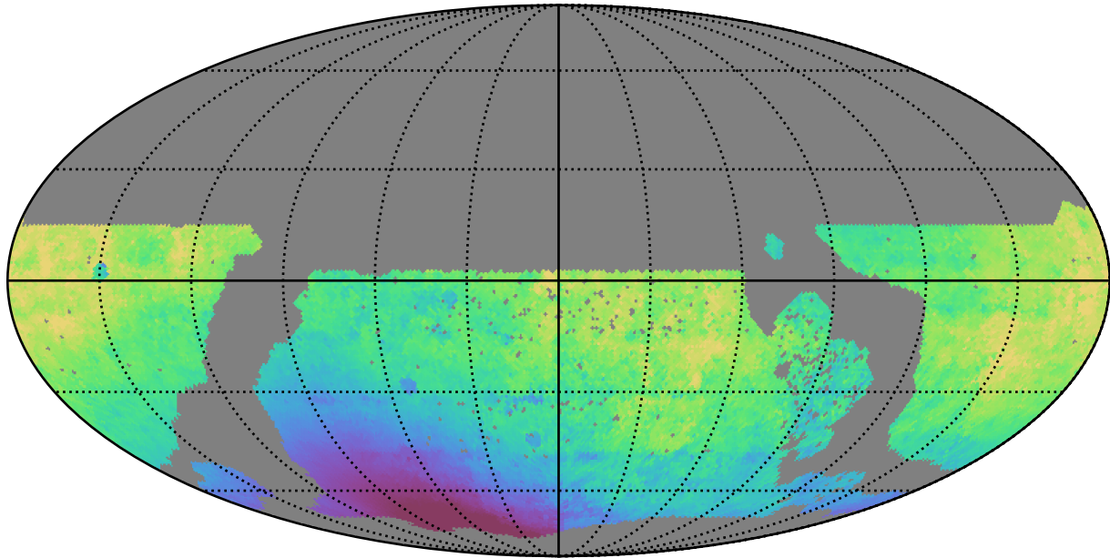
ddf_loaded_fl8_v3.4_10yrs WFD z band: Median solarElong
