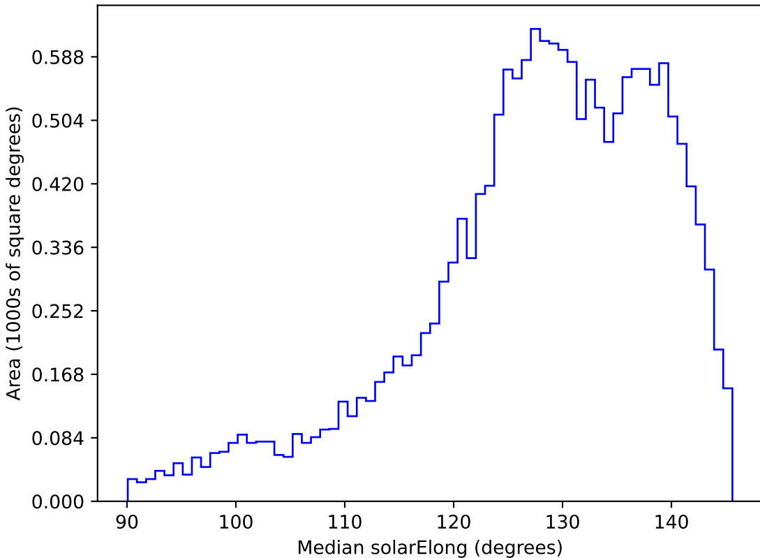
ddf_loaded_fl8_v3.4_10yrs WFD z band: Median solarElong
