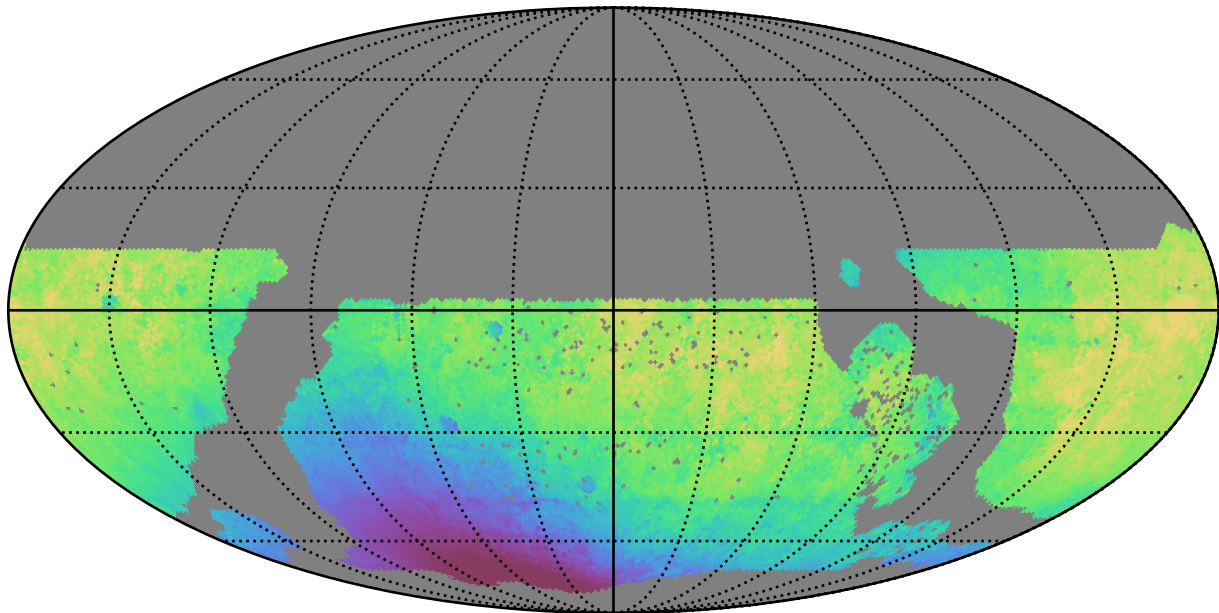
ddf_loaded_fl8_v3.4_10yrs WFD y band: Median solarElong
