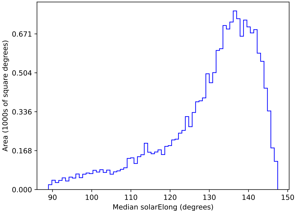
ddf_loaded_fl8_v3.4_10yrs WFD y band: Median solarElong
