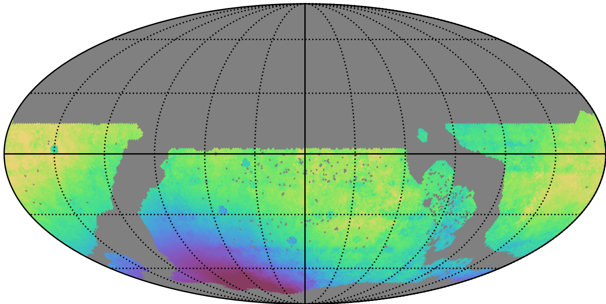
ddf_loaded_fl8_v3.4_10yrs WFD r band: Median solarElong
