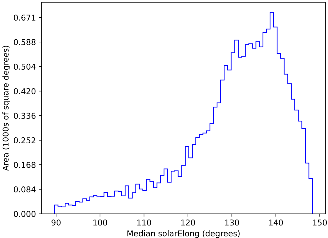
ddf_loaded_fl8_v3.4_10yrs WFD r band: Median solarElong
