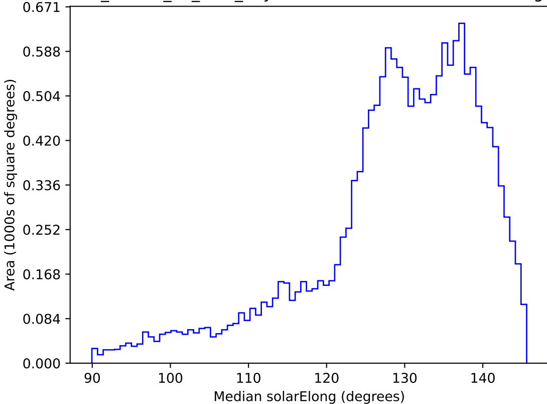
ddf_loaded_fl8_v3.4_10yrs WFD i band: Median solarElong
