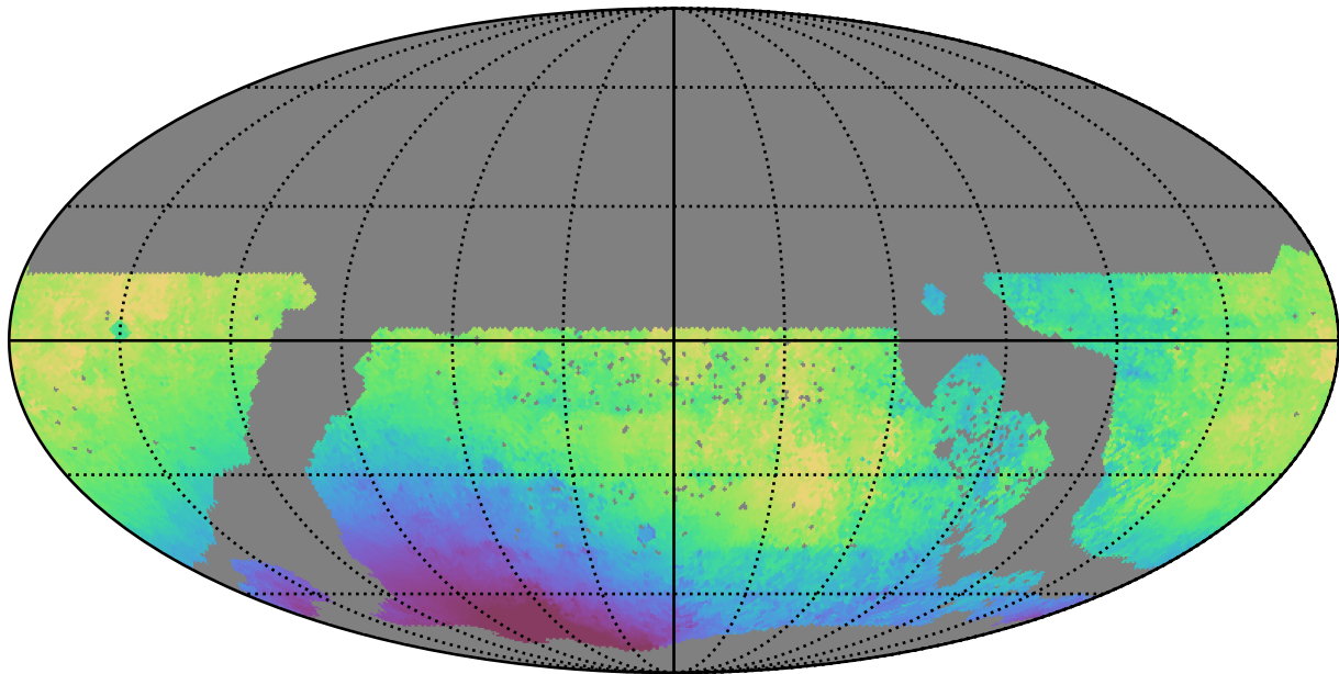
ddf_loaded_fl8_v3.4_10yrs WFD g band: Median solarElong
