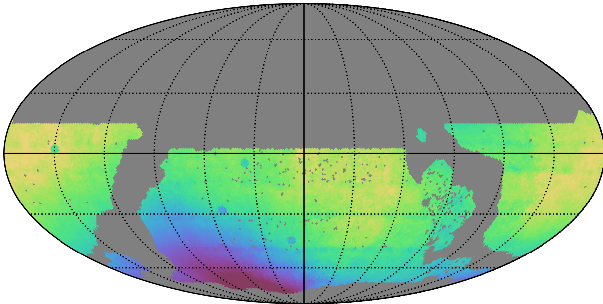
ddf_loaded_fl8_v3.4_10yrs WFD all bands: Median solarElong
