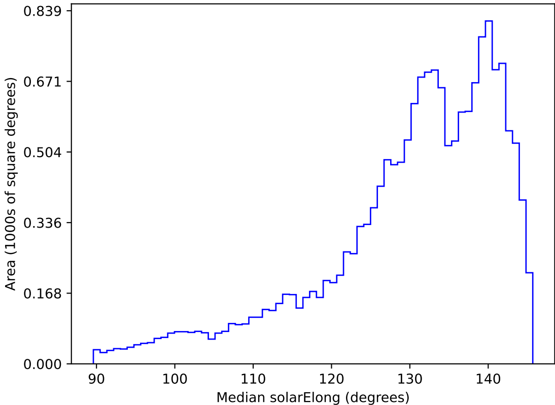
ddf_loaded_fl8_v3.4_10yrs WFD all bands: Median solarElong
