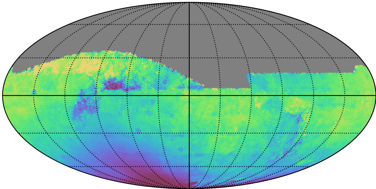
ddf_loaded_fl8_v3.4_10yrs All sky z band: Median solarElong
