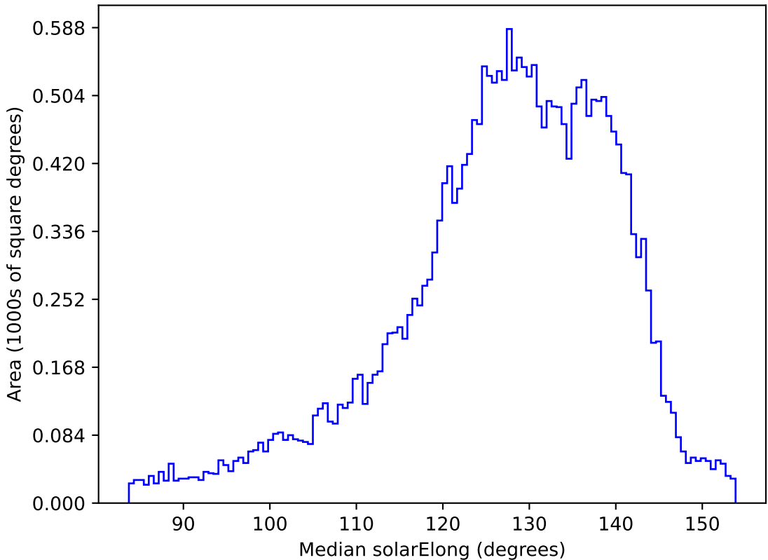
ddf_loaded_fl8_v3.4_10yrs All sky z band: Median solarElong
