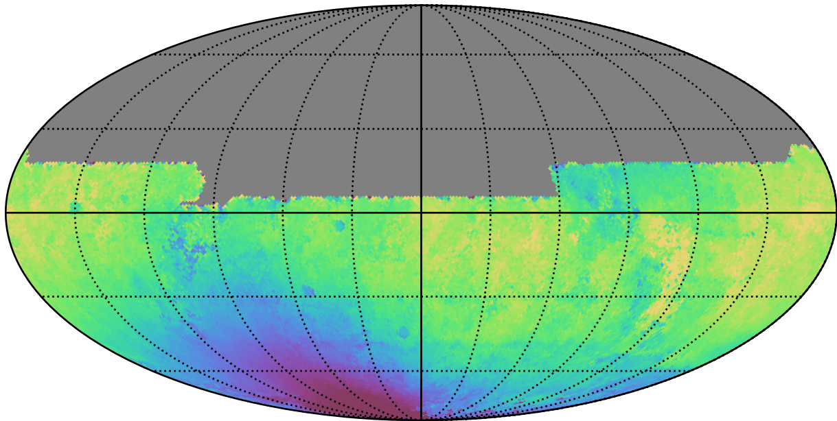
ddf_loaded_fl8_v3.4_10yrs All sky y band: Median solarElong
