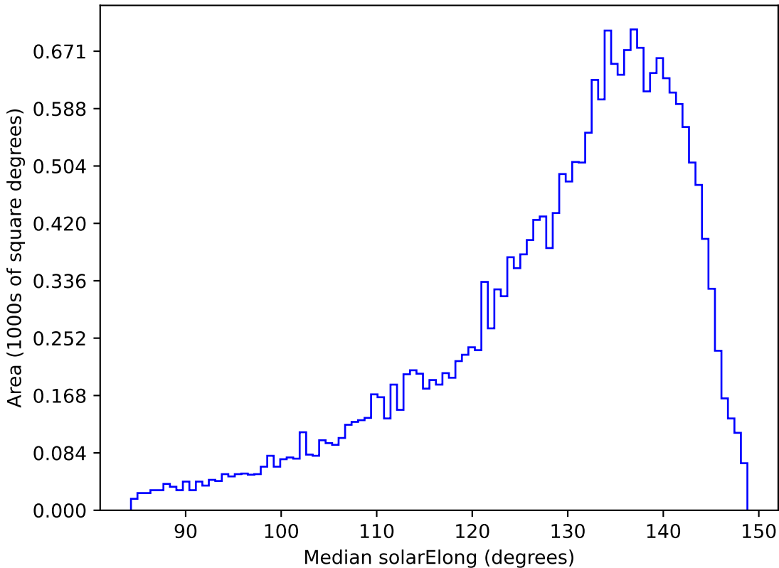
ddf_loaded_fl8_v3.4_10yrs All sky y band: Median solarElong
