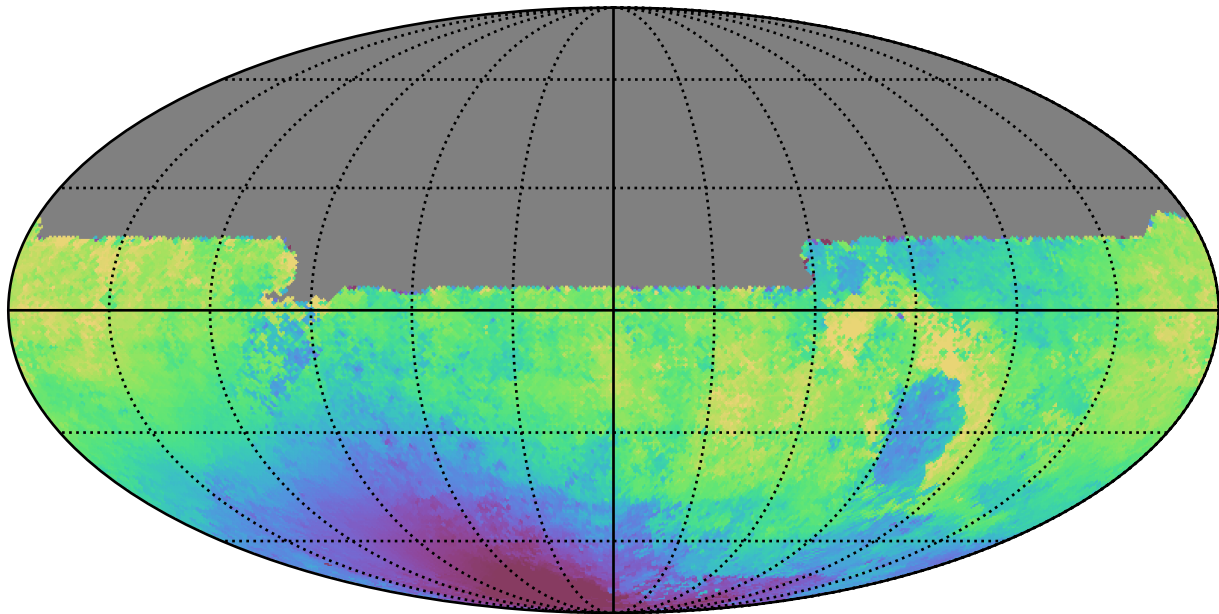
ddf_loaded_fl8_v3.4_10yrs All sky u band: Median solarElong
