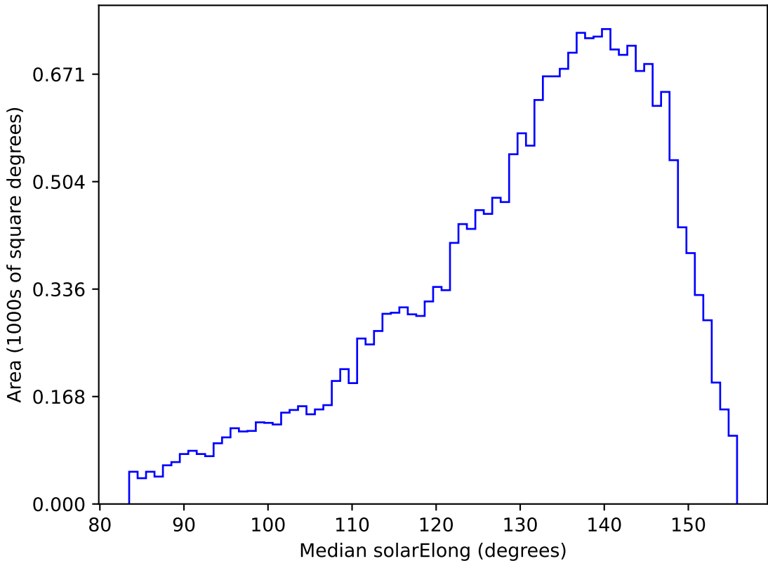
ddf_loaded_fl8_v3.4_10yrs All sky u band: Median solarElong
