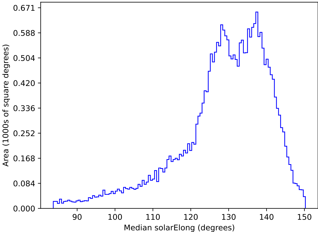
ddf_loaded_fl8_v3.4_10yrs All sky i band: Median solarElong
