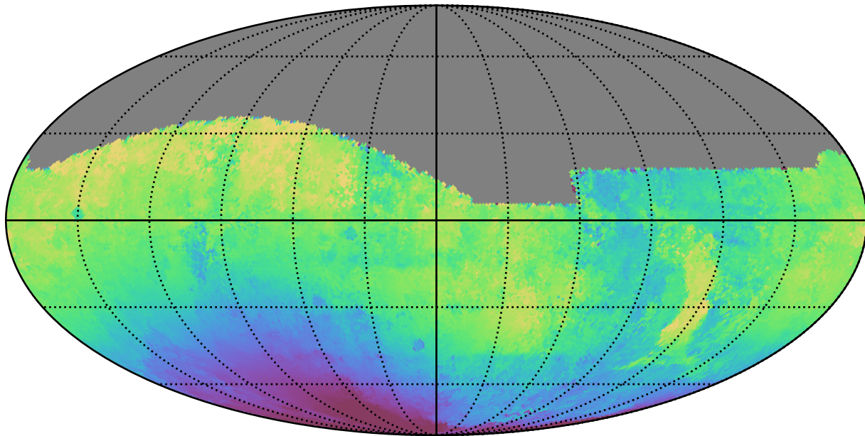
ddf_loaded_fl8_v3.4_10yrs All sky g band: Median solarElong
