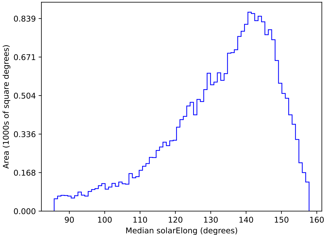
ddf_loaded_fl8_v3.4_10yrs All sky g band: Median solarElong
