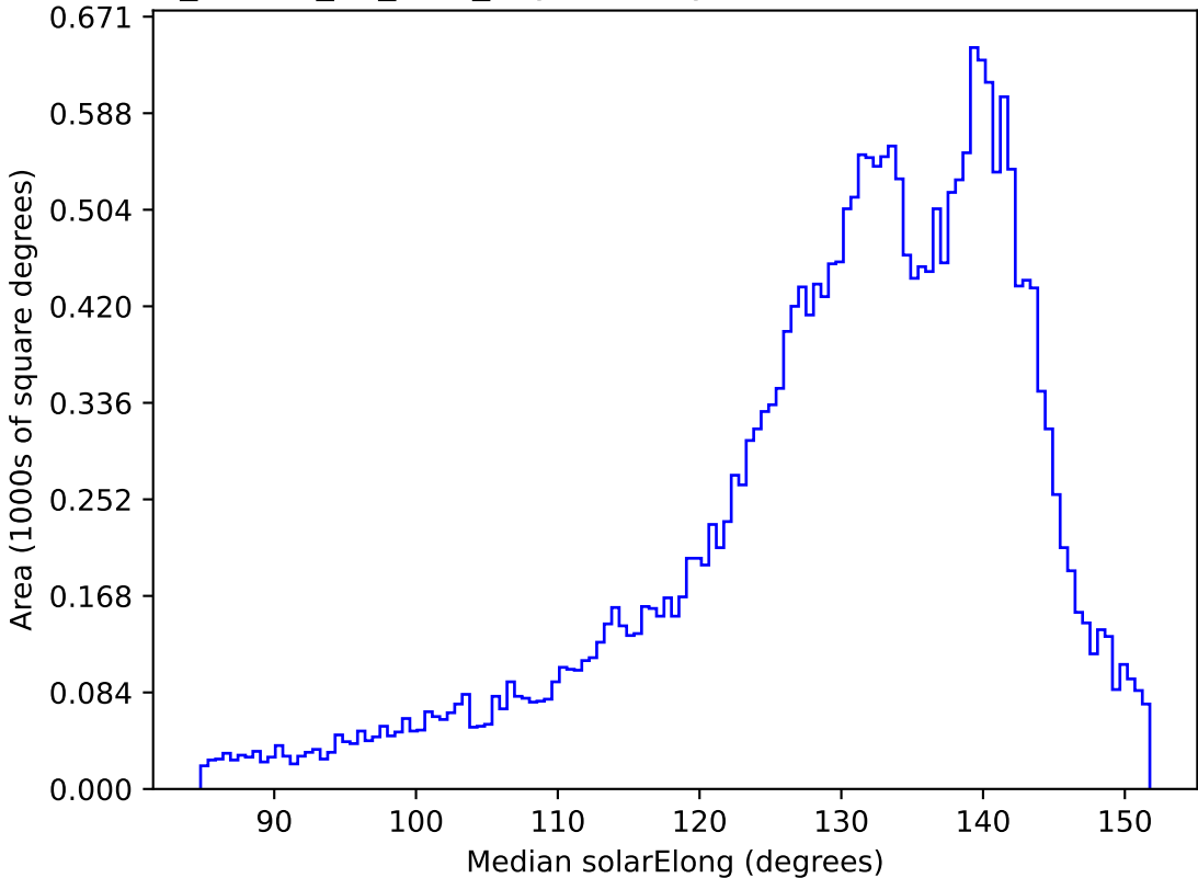
ddf_loaded_fl8_v3.4_10yrs All sky all bands: Median solarElong
