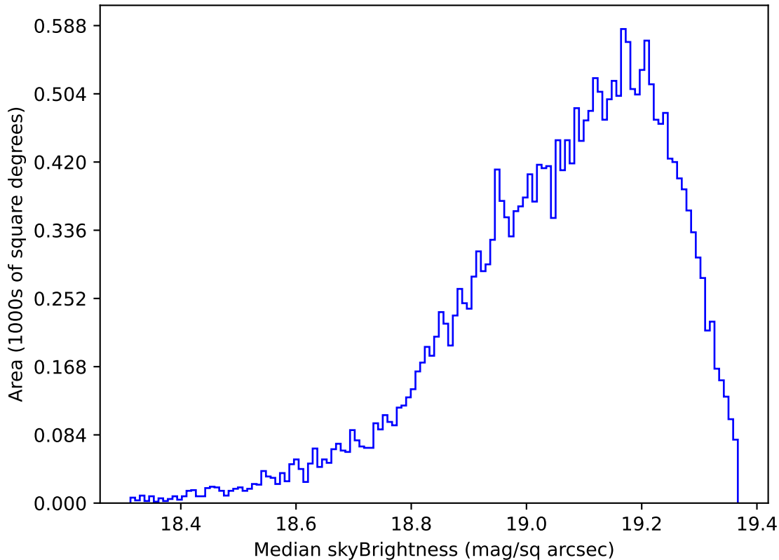
ddf_loaded_fl8_v3.4_10yrs Yr 1 z band: Median skyBrightness
