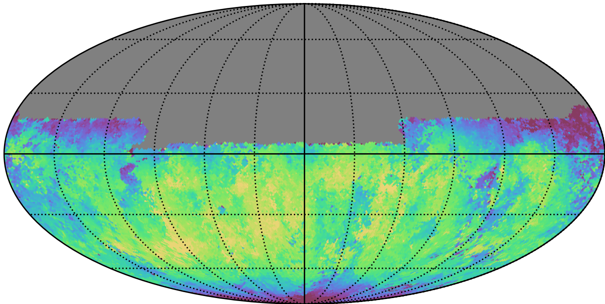
ddf_loaded_fl8_v3.4_10yrs Yr 1 y band: Median skyBrightness
