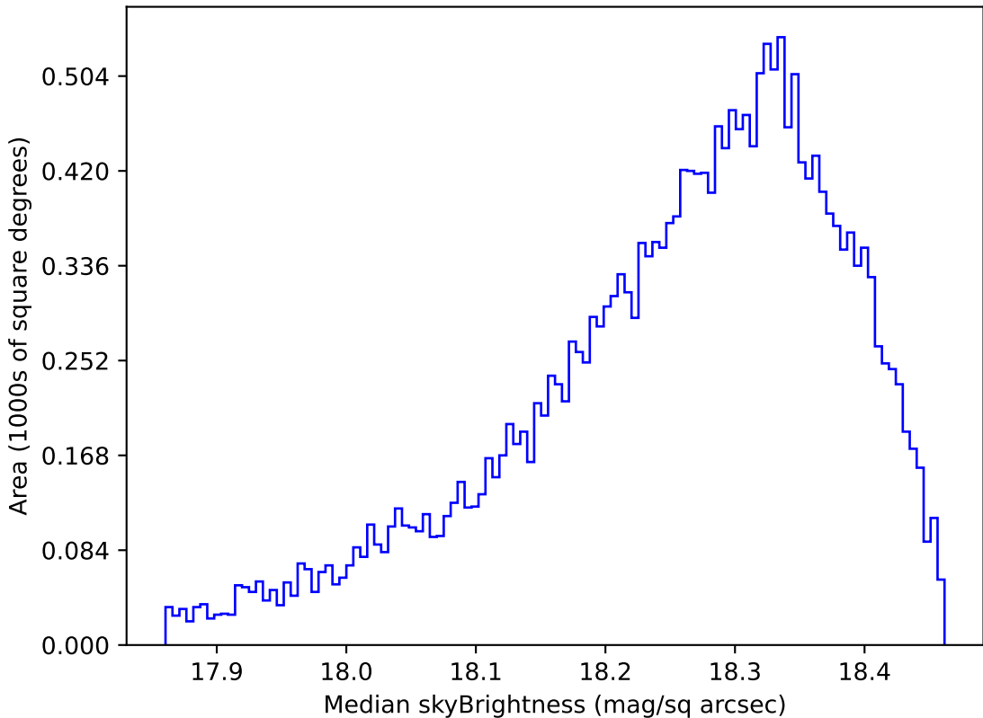
ddf_loaded_fl8_v3.4_10yrs Yr 1 y band: Median skyBrightness
