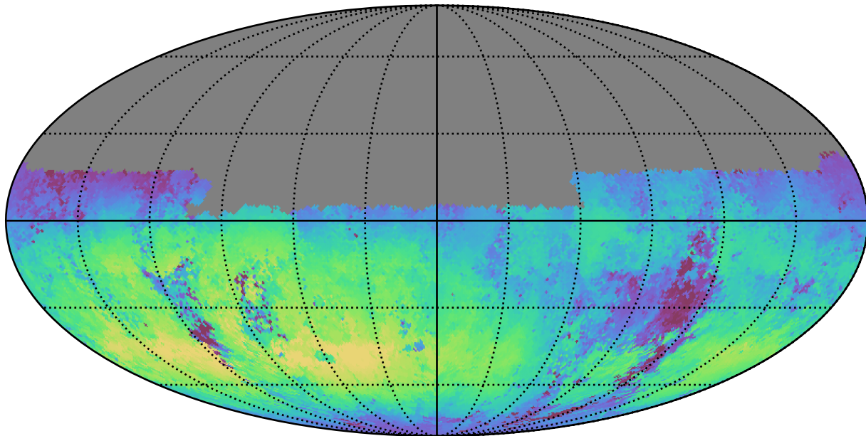
ddf_loaded_fl8_v3.4_10yrs Yr 1 u band: Median skyBrightness
