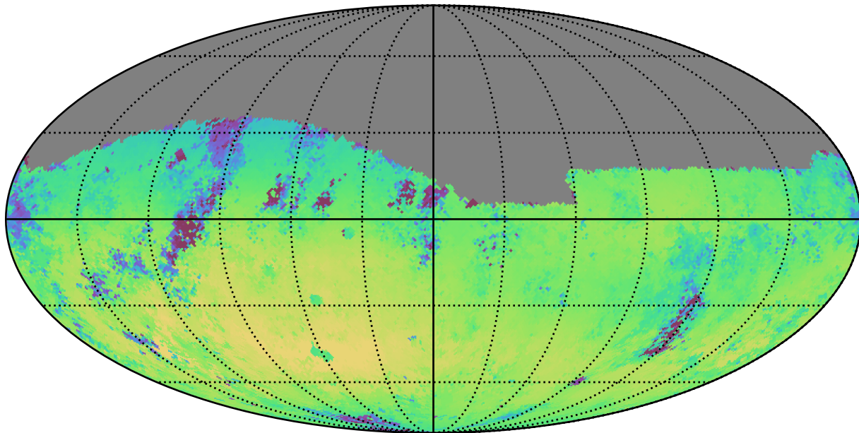
ddf_loaded_fl8_v3.4_10yrs Yr 1 r band: Median skyBrightness
