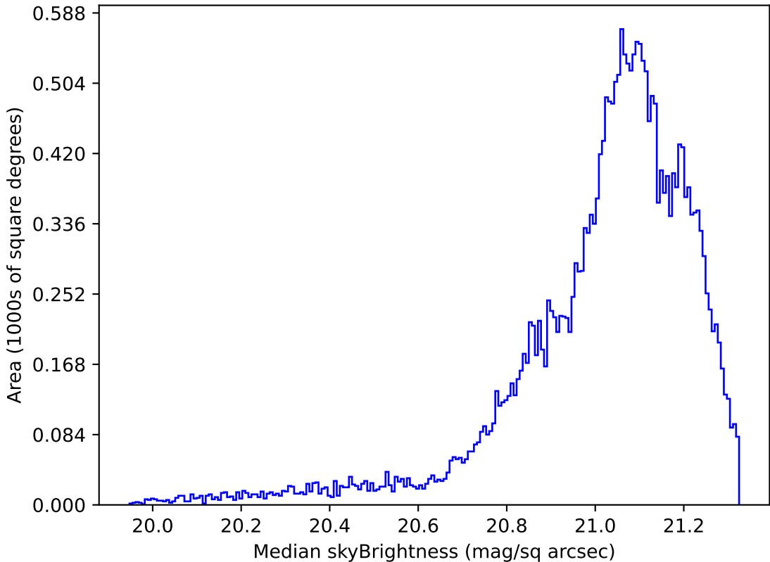
ddf_loaded_fl8_v3.4_10yrs Yr 1 r band: Median skyBrightness
